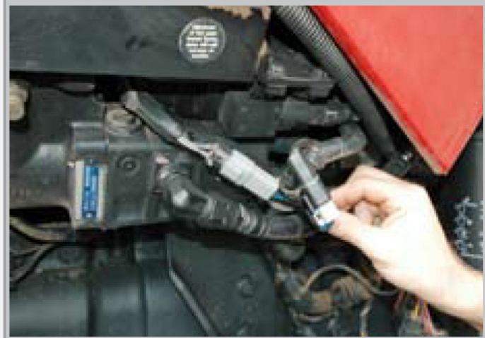
Position of the plug-in connection at the injection pump
